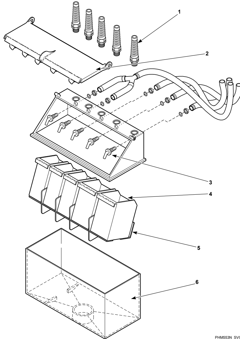
Five Compartment Supply Dispenser (Optional)
